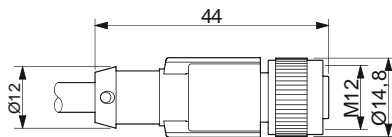
All dimensions in mm
