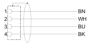
Contact assignment free cable end
