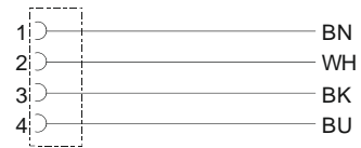
Contact assignment free cable end
