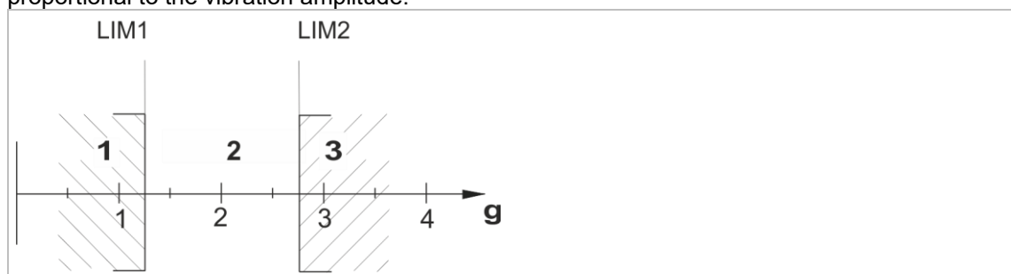
Fig. 2: Window function
