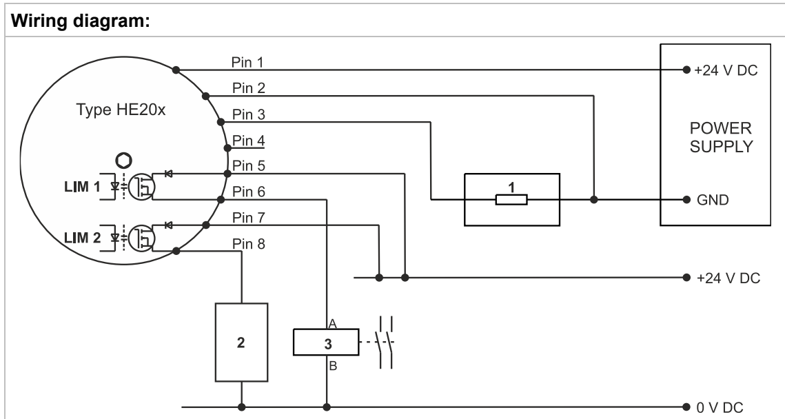
Fig. 1: Wiring diagram
