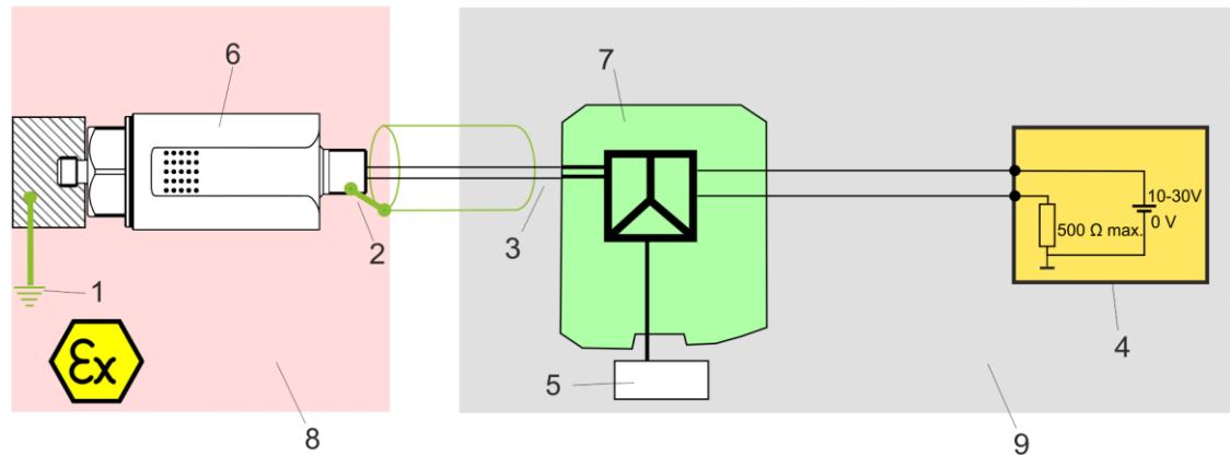
Afb. 12: Ex i aardingsconcept
